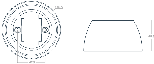
Fitting centres 42.5 mm
