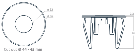
Recessed mount
