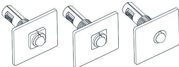
Surface mount** Cut out \varnothing 16 mm
