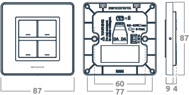
zc-sceneset Dimensions 87 / 87 / 13 mm Mounting centres 64 mm
