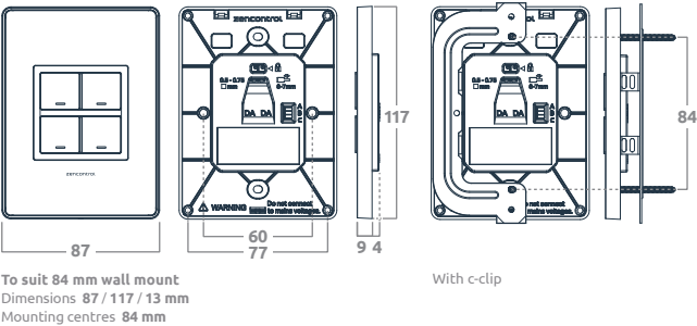
To suit 60 mm wall mount Dimensions 87 / 87 / 13 mm Mounting centres 60 mm
