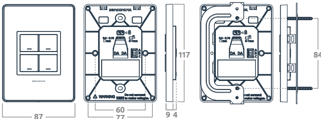
zc-scene-c-a4 Dimensions 87 / 117 / 13 mm Mounting centres 80 mm
